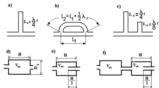
Fig. 2. Types of passive pressure pulsation dampers [4]
