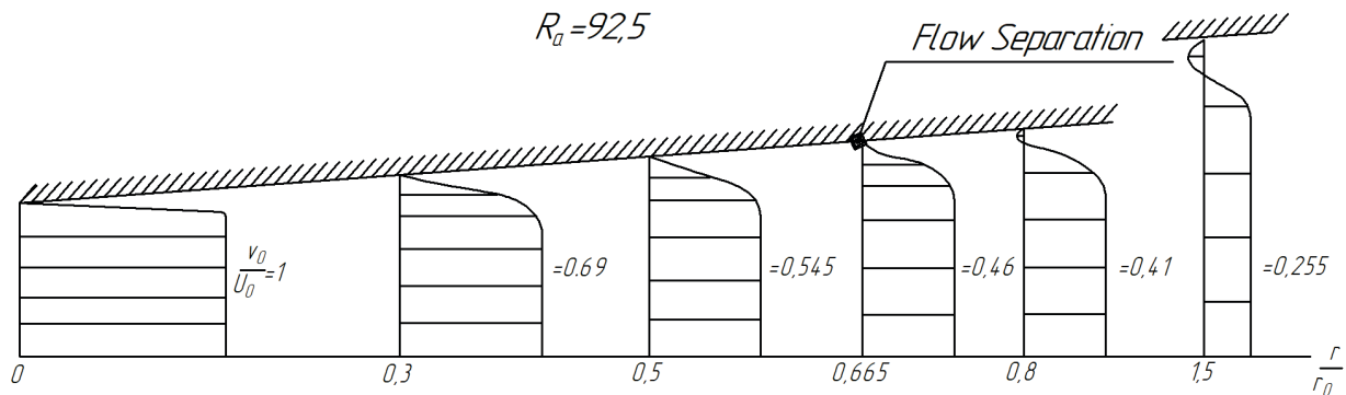
Fig. 1. Velocity profiles in the diffuser [3]
