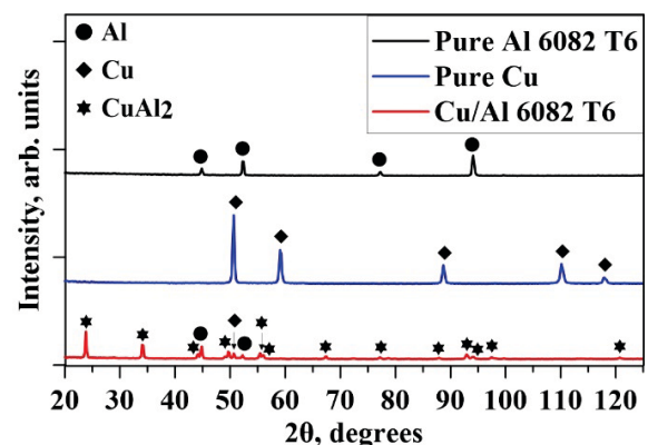
Fig. 4. X-ray patterns of the welded copper-aluminum alloy specimen, pure copper, and pure Al 6082 T6.
