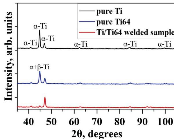
Fig. 7. X-ray patterns of the welded titanium-titanium alloy specimen, pure titanium, and pure Ti64.
