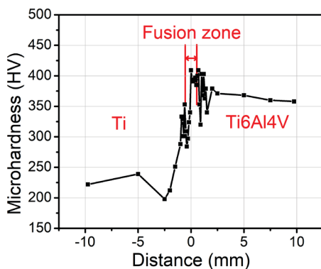
Fig. 9. Distributions of the microhardnesses along the weld cross-section in the middle of the depth of the Ti/Ti6Al4V weld.
